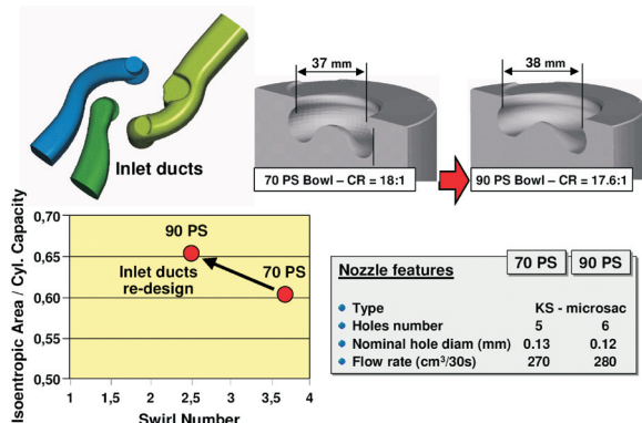
Rys. 8. System spalania Fig. 8. Combustion system
