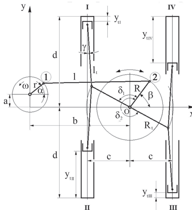
Fig. 2. Basic design parameters of the crank and rocker piston assembly
