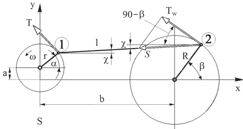
Fig. 7. Schematics for the calculation of the tangential force on the arm of the crankshaft
