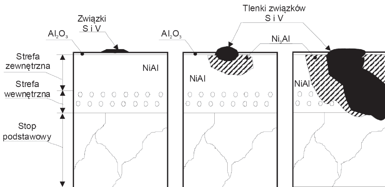
Fig. 6. The mechanism of formation and development of the corrosion of the protective layer of a turbine vane in the Zorya UGT engines
