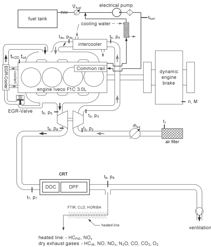
Fig. 2. Engine measuring set-up on the dynamic dynamometer Rys. 2. Schemat stanowiska badawczego
