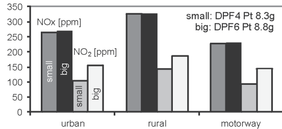
Fig. 9. NO x & NO 2 in ETC with different DPF size, Iveco F1C
