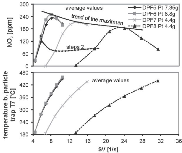
Fig. 10. NO 2 in step test, dependent on exhaust temperature and spacial velocity; DPF's big, Iveco FIC
