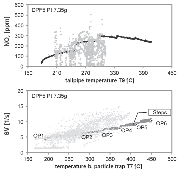
Fig. 11. Comparison of NO 2 , t exh & SV in step test and in ETC, DPF5; Iveco FIC
