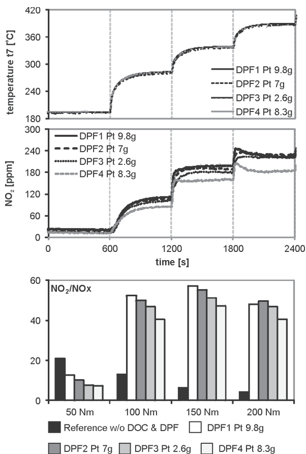
Fig. 5. \text{NO}_2 -production in step-test with different content of Pt in the catalytic coating, smaller DPF's, Iveco engine FIC
