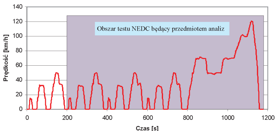
Fig. 1. NEDC driving test with the marked ranges that were subjected to the analysis
