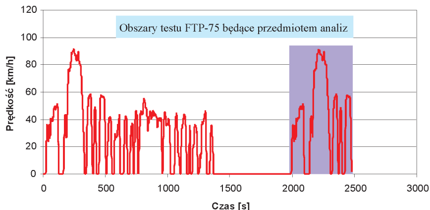
Fig. 2. FTP-75 driving test with the marked ranges that were subjected to the analysis
