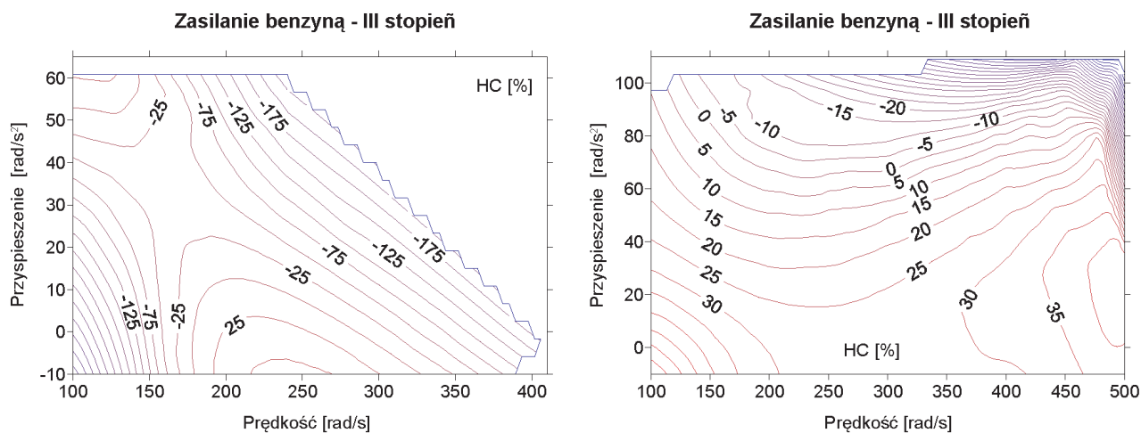
Fig. 7. Errors between the approximation based on the combined data from the FTP-75 and the NEDC and the approximation based on the measurements of only the NEDC and only the FTP-75 for the road emissions of hydrocarbons for gasoline fuelling
