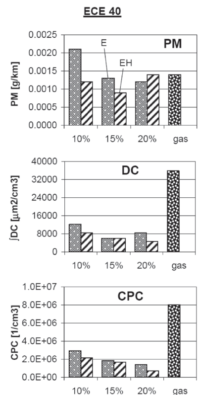
Fig. 17. Particle emissions with different fuels. Honda Zoomer
