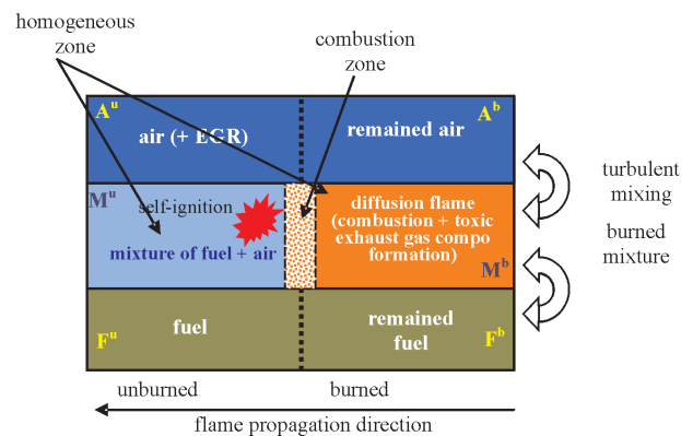
Fig. 2. Zones in the ECFM-3Z model
