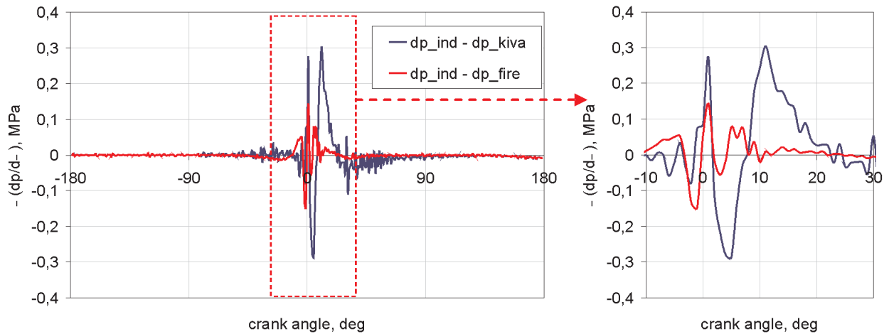
Fig. 8. Difference in pressure increment between the actual values and the values obtained from modelling with the KIVA-3V and the AVL FIRE programs, respectively
