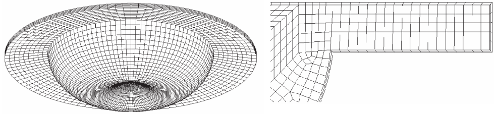
Fig. 3. The computational grid for combustion chamber modelling
