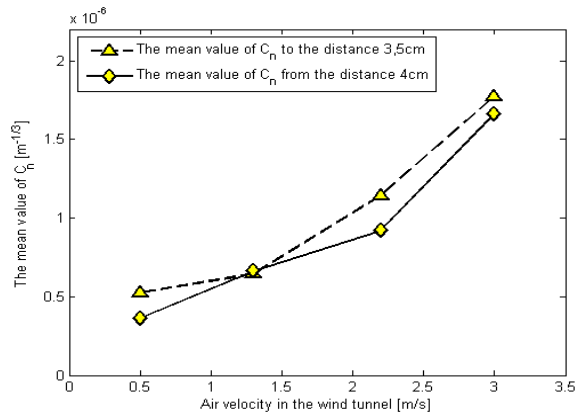
Fig. 8. The C_n parameter mean value dependence on inflowing air velocity in the wind tunnel. The mean values were calculated for two ranges of distances from building model to the laser beam (as described in the legend)
