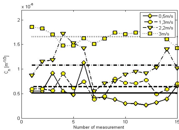
Fig. 5. The C_n parameter versus number of measurement with forced air flow and without the building model in the tunnel. The values of inflowing air velocity in the wind tunnel are specified in the legend
