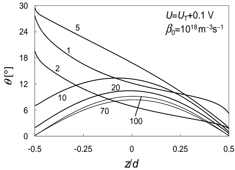
Fig. 3. Director distribution in the deformed layer presented by the angle \theta(z/d) for several anchoring strength W in 10^{-6}\text{ Jm}^{-2} indicated at the curves and for dissociation coefficient \beta_0 = 10^{18}\text{ m}^{-3}\text{ s}^{-1} corresponding to N_0 = 4.7 \times 10^{17}\text{ m}^{-3}
