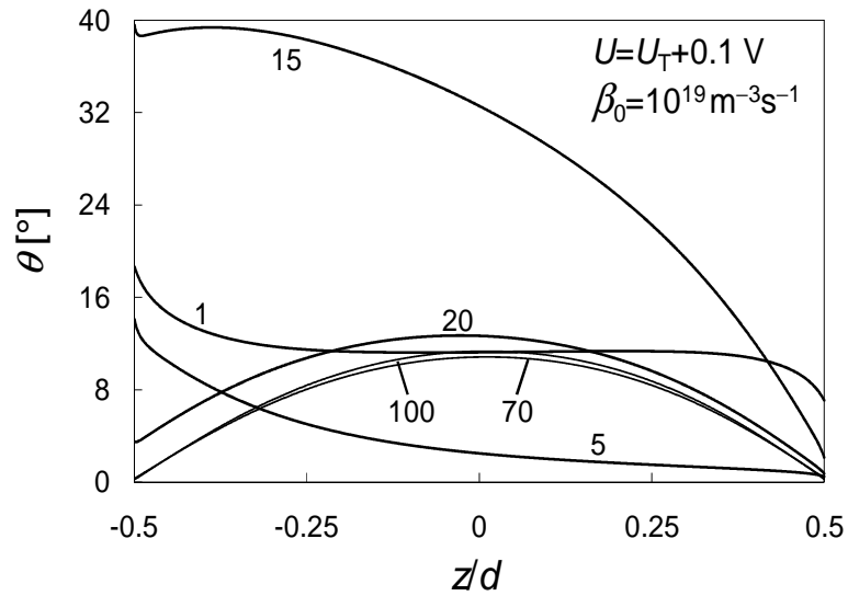
Fig. 4. Director distribution in the deformed layer presented by the angle \theta(z/d) for several anchoring strength W in 10^{-6}\text{ Jm}^{-2} indicated at the curves and for dissociation coefficient \beta_0 = 10^{19}\text{ m}^{-3}\text{ s}^{-1} corresponding to N_0 = 1.5 \times 10^{18}\text{ m}^{-3}
