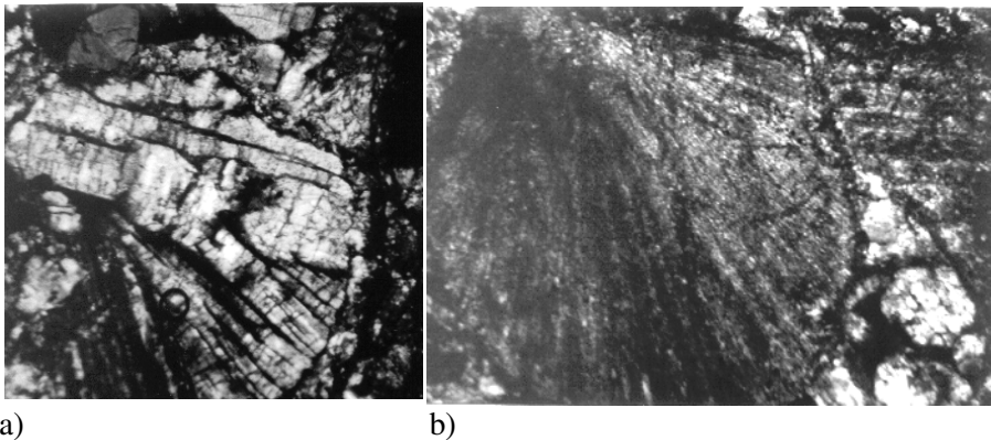
Fig. 11. Optical images of pyroxene chondrules in Gold Basin meteorite: a) Porphyritic pyroxene (PP) chondrule, b) Rimmed radial pyroxene (RP) chondrule. In pyroxene crystals shown in figure (a) shock lamellae parallel running to each other can be seen which indicate shock grade S3 of this chondrite. Field of view: (a) 0.7 mm x 0.7 mm, (b) 1 mm x 0.7 mm
