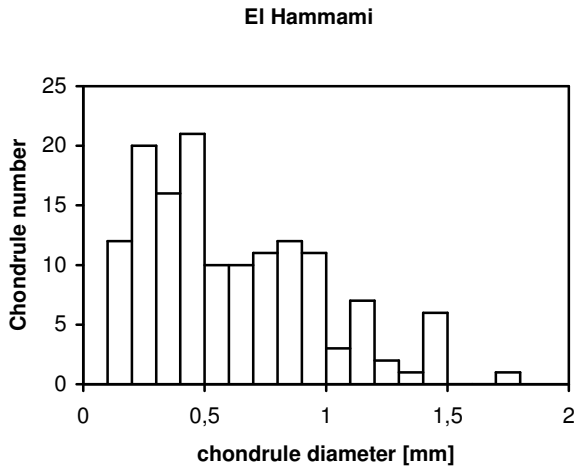
Fig. 14. The histogram of distribution of chondrule size in El Hammami meteorite
