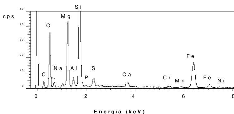
Fig. 2. ED spectrum of Gold Basin meteorite revealing elements contributed to the mean bulk composition of the meteorite
