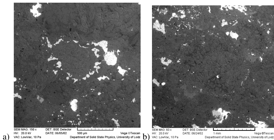
Fig. 6. Electron microscope (BSE) images of olivine chondrules and matrix in Gold Basin meteorite. Notice various minerals present in this chondrite. White areas are Fe-Ni phases, grey represent troilite, and dark areas are mostly olivines and pyroxenes
