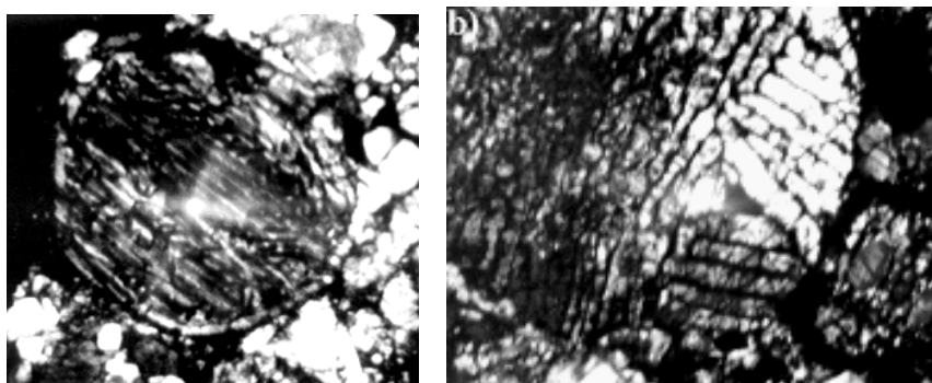
Fig. 12. Optical images of barred olivine (BO) chondrules: (a) El Hammami, (b) Gold Basin. Field of view: (a) 0.7 x 0.7 mm, 0.9 x 0.7 mm
