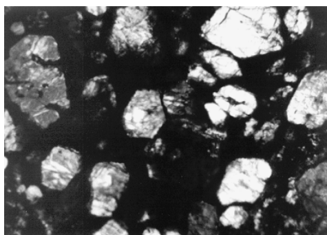
Fig. 15. Euhedral olivine and pyroxene crystals in the matrix of Gold Basin meteorite revealing the porphyritic structure of this region of the meteorite. Field of view 1 mm x 0.7 mm
