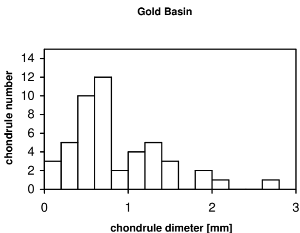
Fig. 13. The histogram of distribution of chondrule size in Gold Basin meteorite
