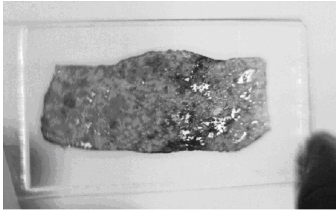
Fig. 10. Thin section of Gold Basin meteorite. White patches are Fe-Ni phases seen in reflected light
