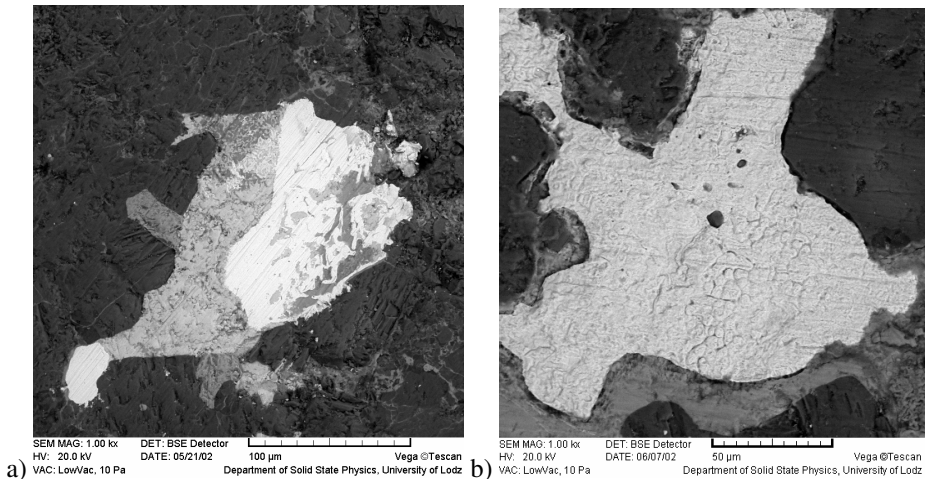
Fig. 5a,b. BSE images of matrix of El Hammami meteorite showing various minerals present in this multicomponent meteorite piece. White areas are Fe-Ni phases, grey are troilite, and dark areas are mostly olivines and pyroxenes, the major minerals of chondrites
