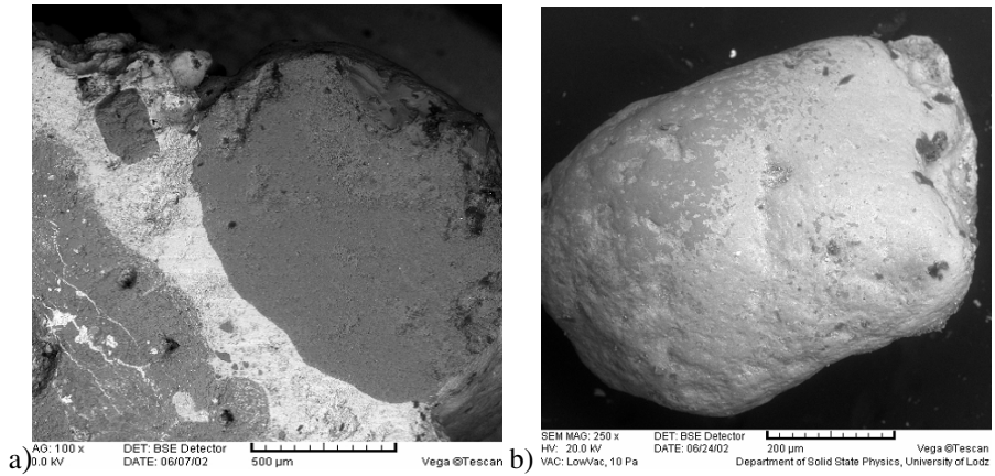
Fig. 7. BSE images of chondrules and the matrix of El Hammami meteorite. (a) orthoclase chondrula with the magnetite rim. The rim is surrounded by kamacite, (b) Silica chondrula
