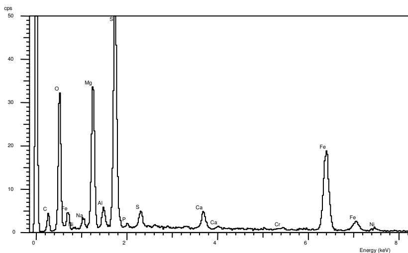
Fig. 3. ED spectrum of El Hammami meteorites revealing elements contributed to the mean bulk composition of the meteorite
