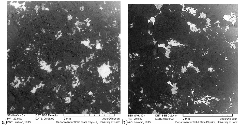
Fig. 4. BSE images of El Hammami and Gold Basin meteorites. FeNi phases kamacite and taenite are seen as white spots, troilite as grey, and silicate minerals are represented by dark colours. Chondrules, chondrule rims and the matrix can be seen in these images. (a) El Hammami, (b) Gold Basin
