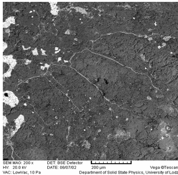
Fig. 8. Electron microscope (BSE) image of the matrix of El Hammami meteorite showing troilite (FeS) veins
