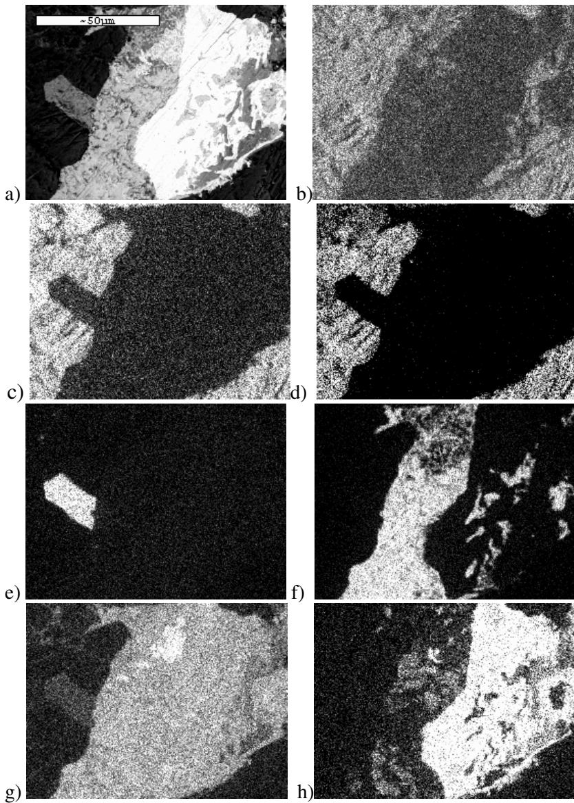
Fig. 9. Distribution (chemical map) of elements in El Hammami meteorite: a) BSE image, b) O, c) Mg, d) Si, e) Cr, f) S, g) Fe, h) Ni distribution. White color shows a high concentration of the element, dark absence of the element in a given region of meteorite. Field of view: 0.125 mm x 0.10 mm
