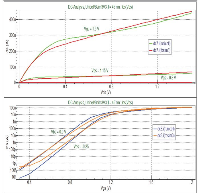
Fig.2. I_{ds}(V_{ds}, V_{gs}) and I_{ds}(V_{gs}, V_{ds}) characteristics comparisons with UNICELL 3 and BSIM3V3, L=45 nm
