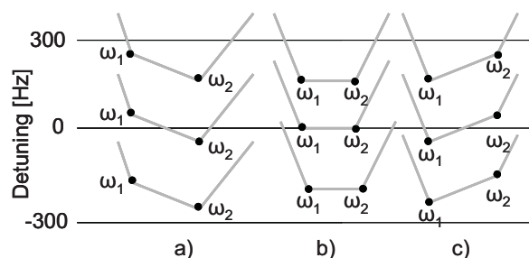
Figure 5. The possible states of the cavity detuning curves (a – without compensation, b – with compensation, c – overcompensation).
