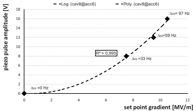
Figure 6. The second order polynomial fitting of piezo compensation pulse amplitude versus set point gradient for cavity 8 in ACC6. The compensated Lorentz force detuning over the flattop region is collected close to each piezo pulse amplitude measurement.
