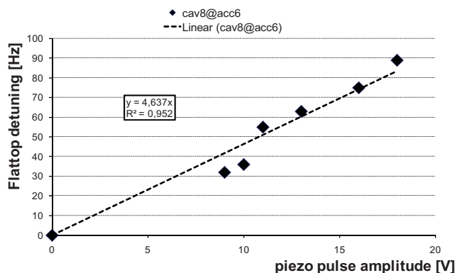
Figure 3. The linear function fitting of compensating Lorentz force detuning over the flattop region versus piezo pulse amplitude in cavity #8 in ACC6.
