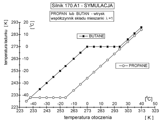
Fig. 4. Expected values of charge temperature of the 170.A1 engine fuelled with pure propane or pure butane, air excess coefficient \lambda = 1
