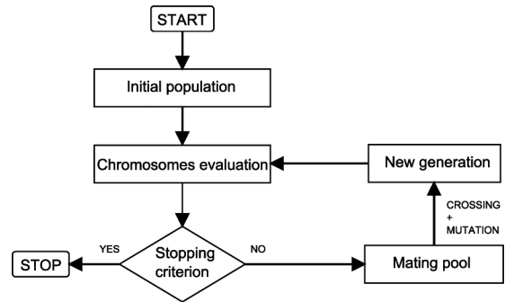
Fig. 4. Diagram of genetic algorithm operation
