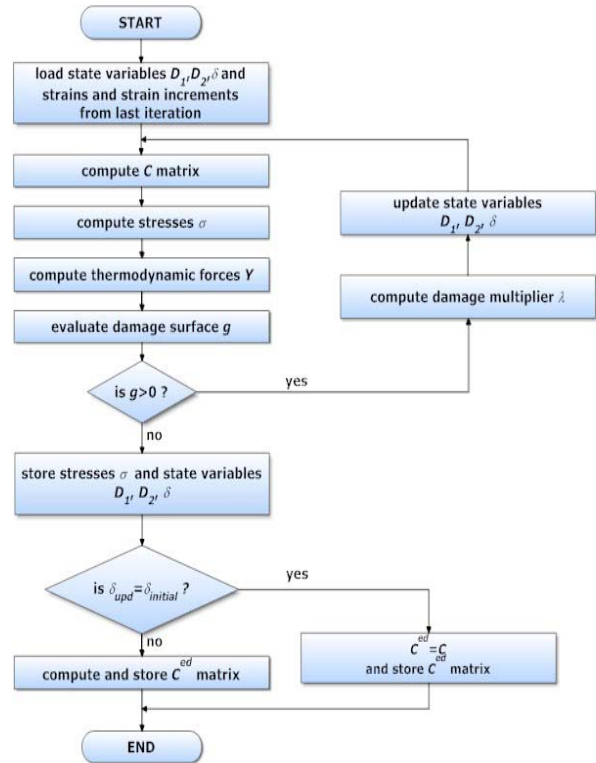
Figure. 2 Flowchart of numerical damage analysis of thin plates
