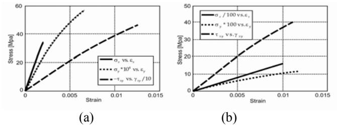
Figure. 3 Stress and strain evolution for material M30/949 in (a) IP 1, (b) IP 872
