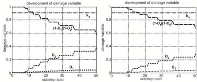
Figure.6 Damage variables evolution for material M30/949 in (a) IP 868, (b) IP 872
