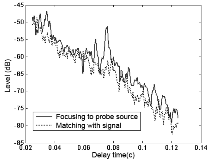
Fig.7 Echogram corresponding matching with signal of source (dotted line) and focusing to probe source near a tone pier (a continuous line)
