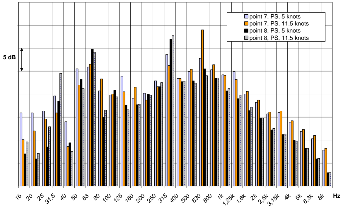
Fig.9 Noise levels at distance 1 m from main gear and shaft generator area (PS) for 1/3 octave bands
