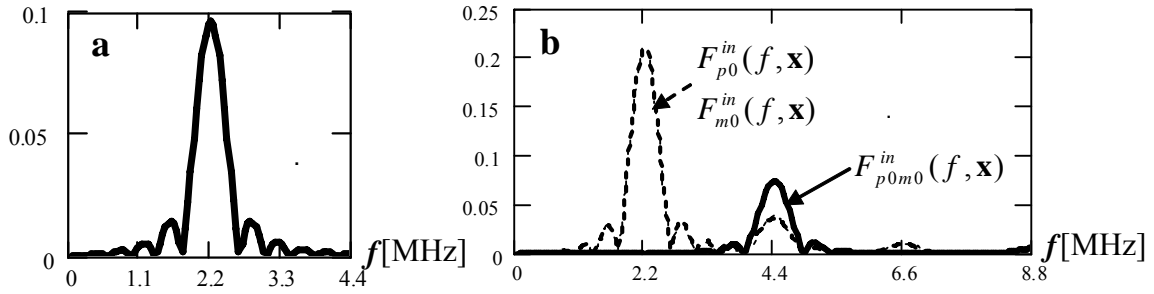
Fig.1 Moduli of the Fourier spectra for the PI method. (a) Fourier spectra of the pulses from the Eq.(2). (b) Results of nonlinear propagation of pulses as in Eq.(2) for PI-near physical focus \mathbf{x}=(0\text{mm}; 40\text{mm}) . F_{p0}(f, \mathbf{x}) , F_{m0}(f, \mathbf{x}) -module of Fourier spectra of incident pulses-dashed lines;
