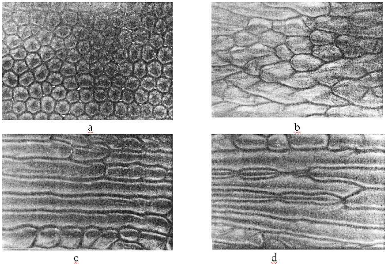
Fig.2 Photo images of the silicon oil heated from below for immovable air (a), immediately after starting of the wind blowing (b, V=12\text{ cm/c} ), and at the steady wind velocity V_o = 160\text{ cm/s} (c), and 180\text{ cm/c} (d)
