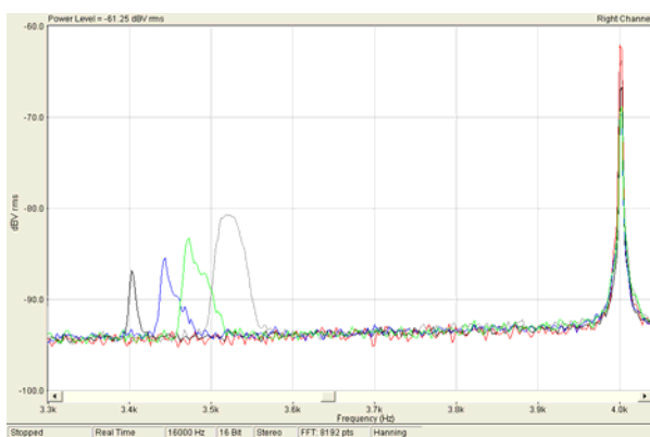
Fig.4 Spectra of the scattered sound
