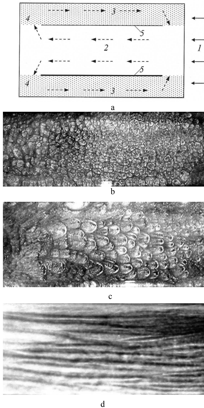
Fig.1 Sketch of the experimental setup (a) and images of the fluid surface for immovable air (b), immediately after starting of the wind blowing (c), and at the steady wind velocity V_0 = 1.5 m/s (d). Designations in (a) are 1- forward air flow, 2 (dashed arrows) - wind-driven fluid flow, 3 (dashed arrows) - counter fluid flow, 4 (shaded fields) - horizontal screens above the counter flow, 5 - vertical screens delimiting the accompanying and counter flows
