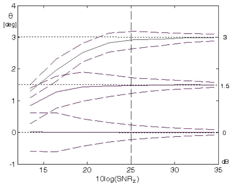
Fig.7. Mean values and standard deviations of bearings in the function of the output signal to noise ratio ( \theta=0^\circ , \theta=1.5^\circ , \theta=3^\circ )
