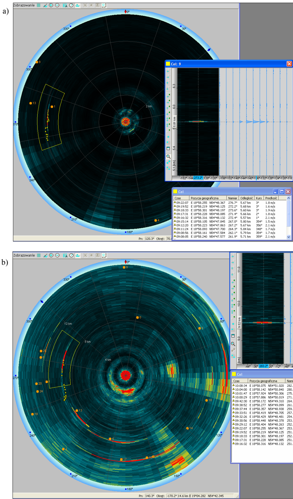
Fig.3 The examples of sonar display with reverberation interference background level made stationary for submarine tracking a) 5.67 km away at 273° bearing and ship's head at 49°; b) 9.94 km away at 282° bearing and ship's head at 306°
