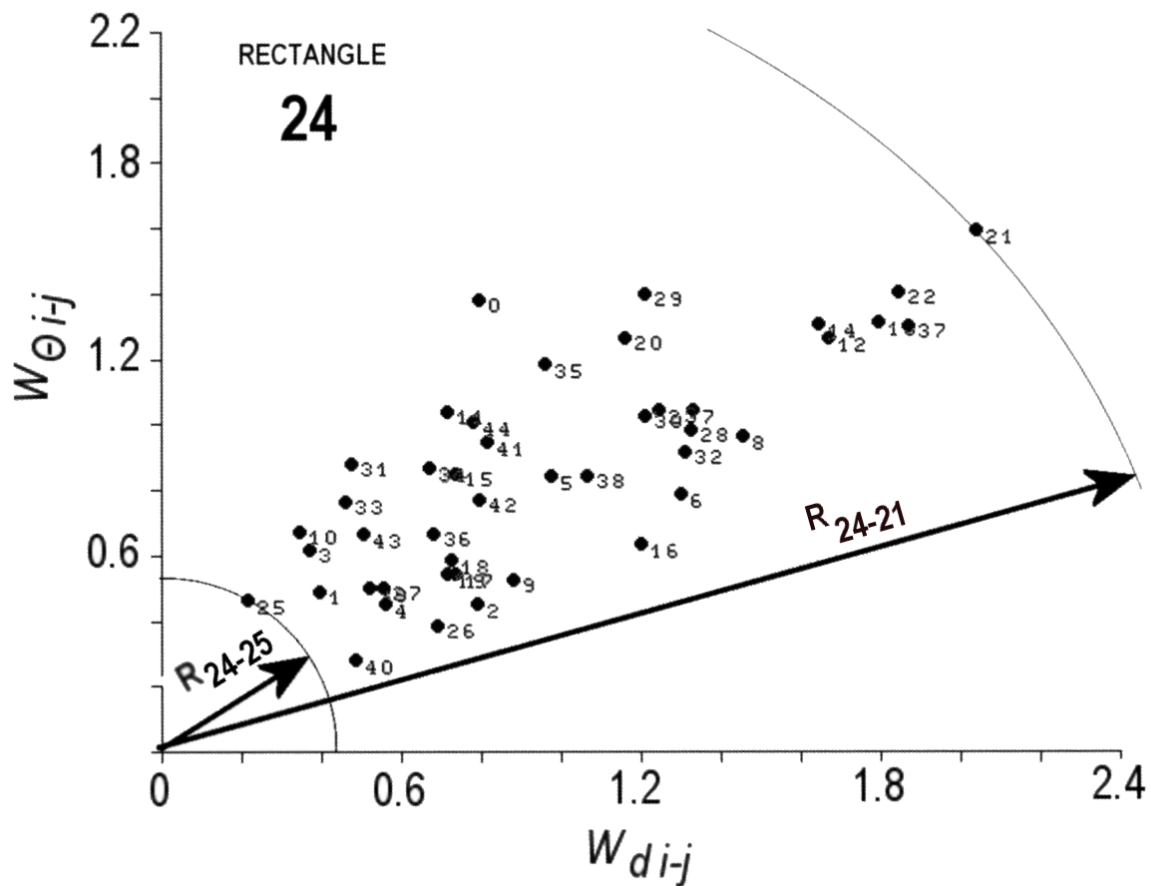
Fig.6 Comparison of acoustic characteristics of selected statistical rectangle (24 in this example) to all remained areas. R_{24-25} – distance between rectangle 24 and 25, R_{24-21} – distance between rectangle 24 and 21. Numbers correspond to rectangle in compared pair
