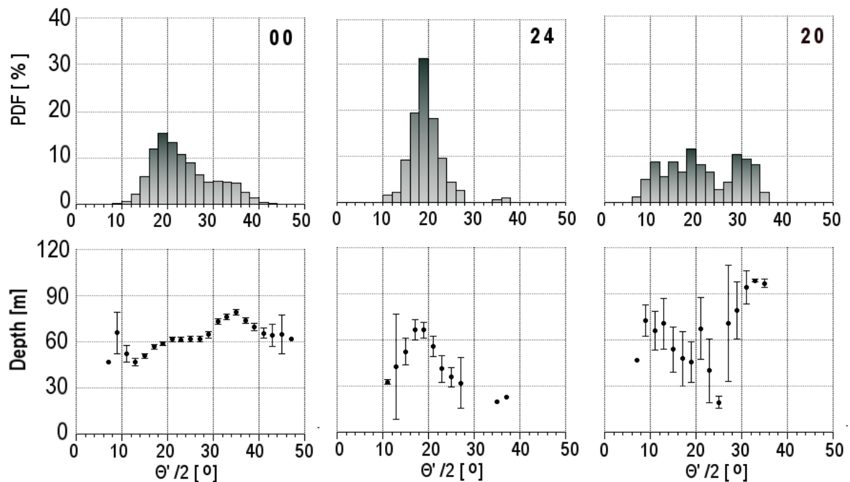
Fig.3 Examples of PDF distributions of \Theta'/2 and average depths for each statistical intervals for the whole southern Baltic (00) and two characteristic rectangles 24 and 20 (see Fig.2)
