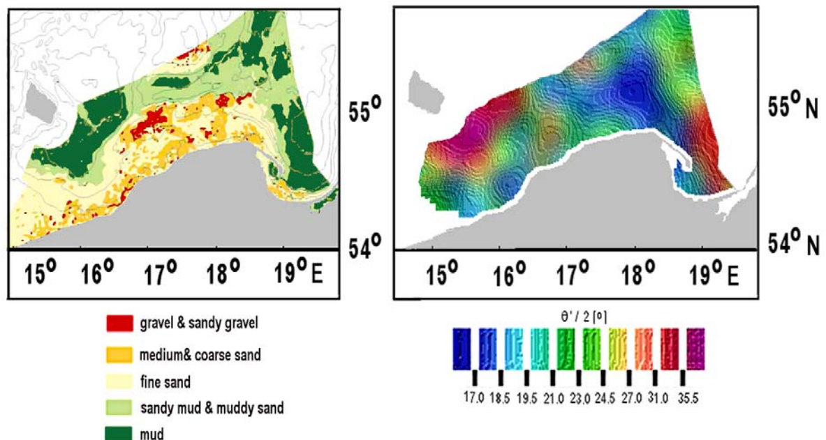
Fig.7 Comparison of geological and acoustic ( \Theta'/2 measurements) classification of the southern Baltic seabed
