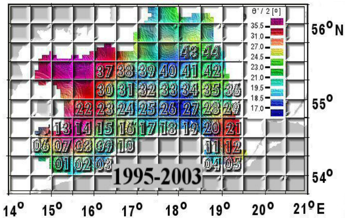
Fig.2 Charts of both parameters: bottom depth and \Theta' / 2 values, evaluated from data collected. Division of the analysed area into standard rectangles 01-44
