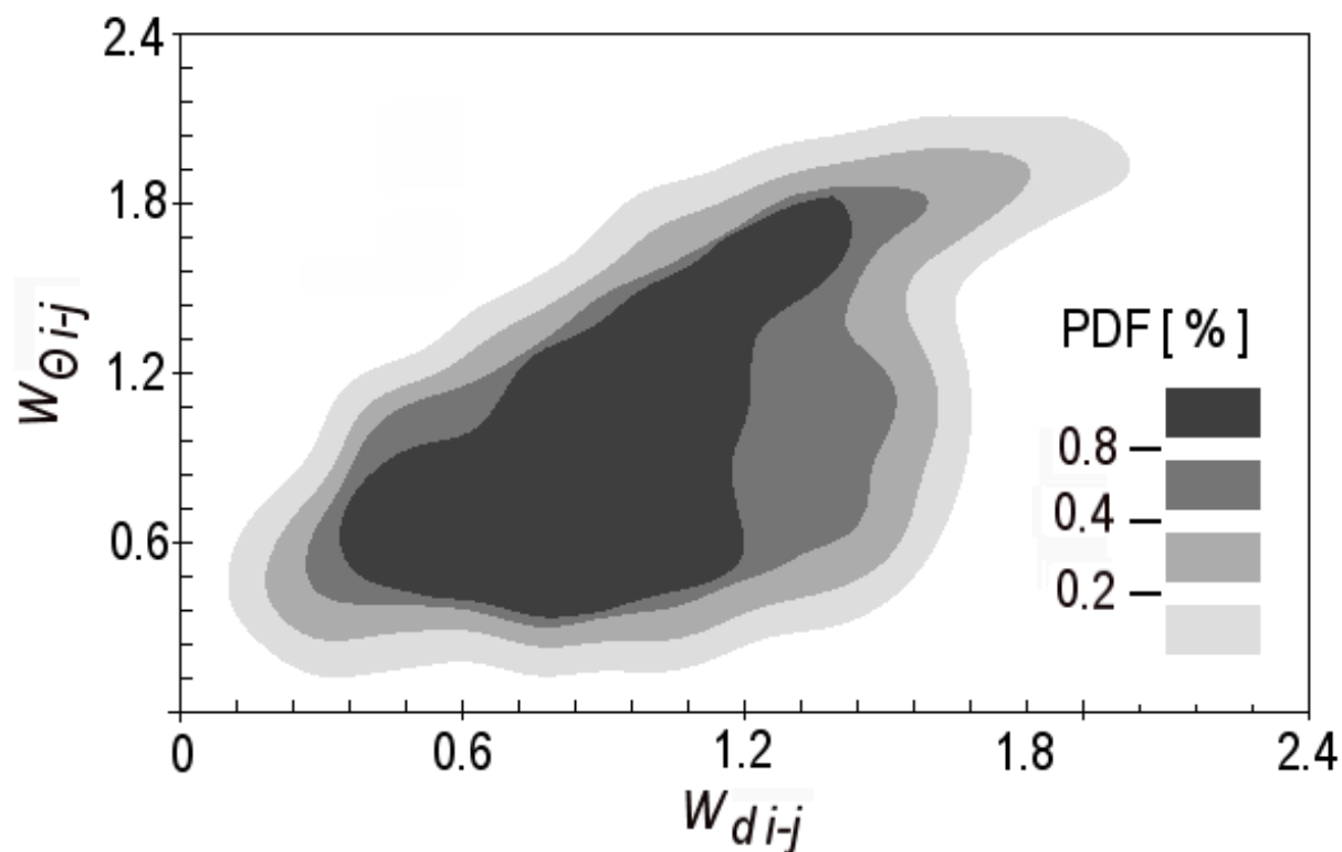
Fig.5 Probability density distribution of factors W_{di-j} and W_{\Theta i-j} calculated for pairs characterizing 44+1 statistical rectangles of southern Baltic
