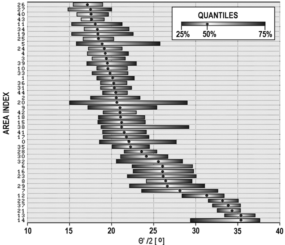
Fig.4 Medians and quantiles of \Theta'/2 per each statistical rectangle (area index), ordered in relation to median values of \Theta'/2
