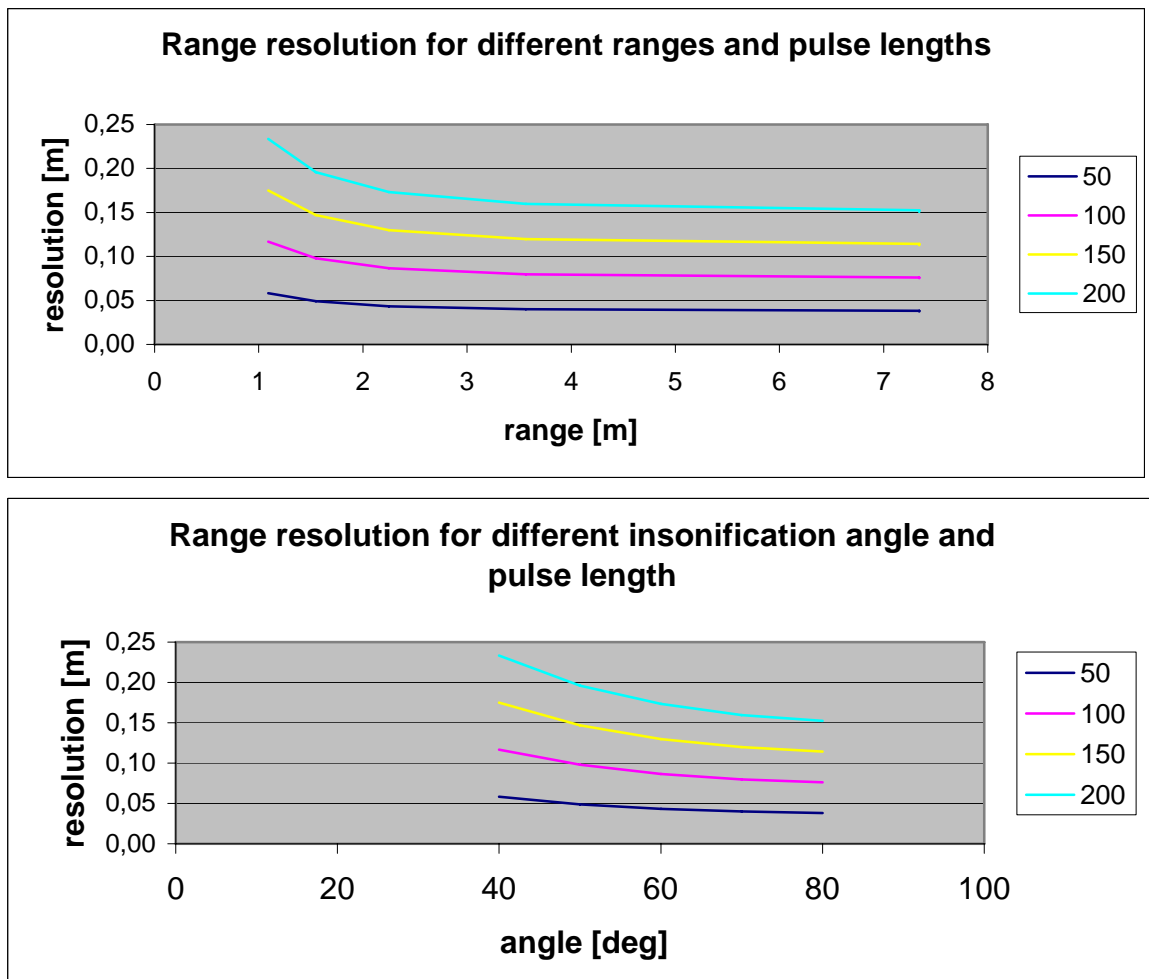
Fig.6 Depth resolution for different ranges [m] , insonification angle [°] and pulse length [ \mu\text{s} ]
