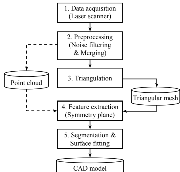
Fig. 1. Typical flow of reverse engineering [6]
