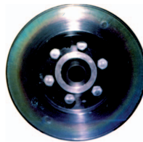
Photo 4. Image of an overheated and seized viscous torsional vibration damper, acc. tests made by the DAMPOL
