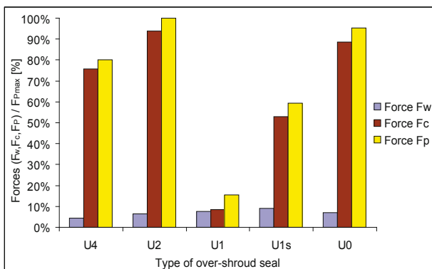
Fig. 15 Values of the blade-ring forces F_w (blue), pressure forces F_c (brown), resultant force F_p (yellow), at 20kPa inlet overpressure and 566 rad/s rotor angular frequency
