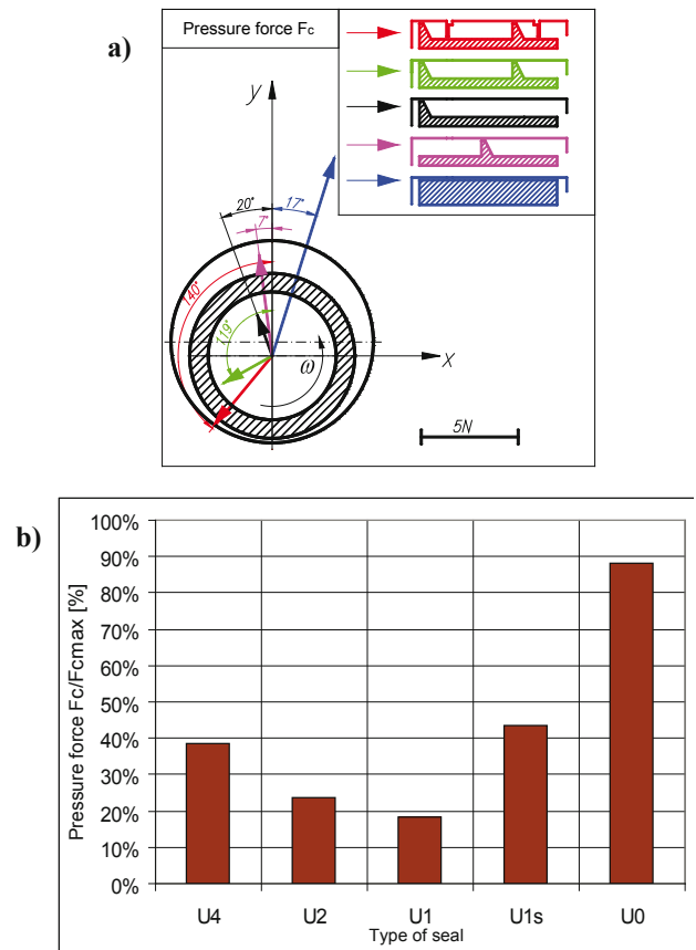
Fig. 11 Vectors, (a), and values, (b), of the pressure force FC occurring in the investigated seals for viscous working medium and the shroud wall angular frequency equal to 566 rad/s (the force values are related to that which occurs in the U0 seal of motionless shroud)
