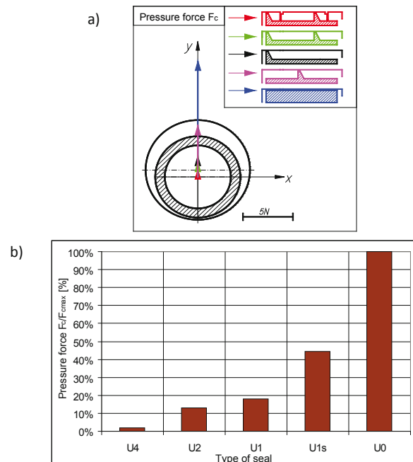
Fig. 9 Vectors, (a), and values, (b), of the pressure force F_c , occurring in the investigated seals (the force values are related to that which occurs in the seal U0) (red colour stands for the seal U4, green colour – the seal U2, black colour – the seal U1, violet colour – the seal U1s, blue colour – the seal U0)
