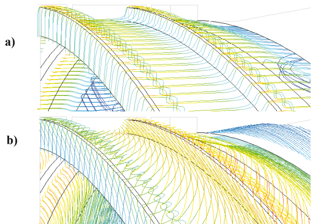
Fig. 12 Pathlines of viscous working medium flowing through the seal U4: (a) in the case of motionless shroud, (b) in the case of rotating shroud with the angular frequency equal to 566 rad/s
