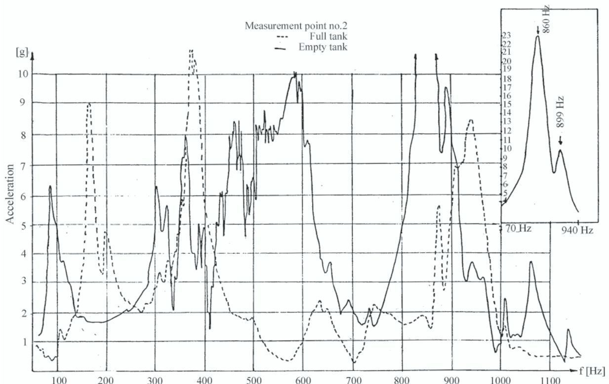
Fig. 4. Run of vibrations at the measuring point 2
