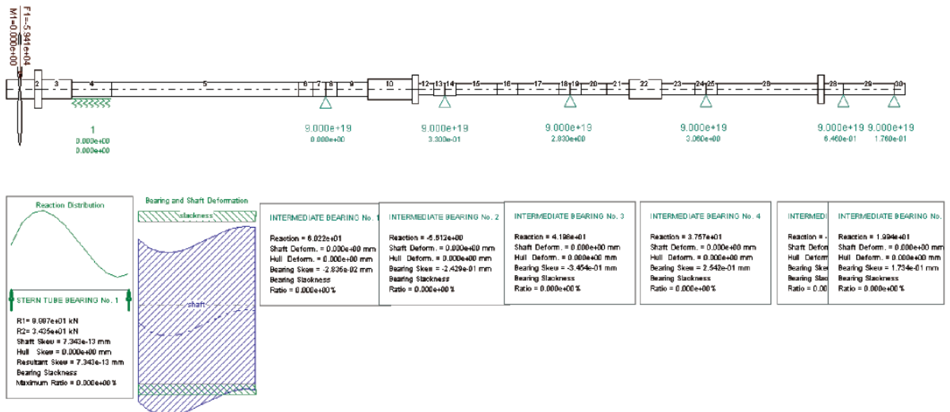
Fig. 16. Design shaft line alignment and reactions
