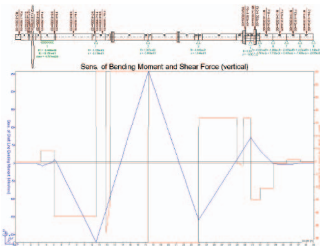
Fig. 14. Influence coefficients of bending moments and shear forces under the influence of vertical movement of aft intermediate bearing
