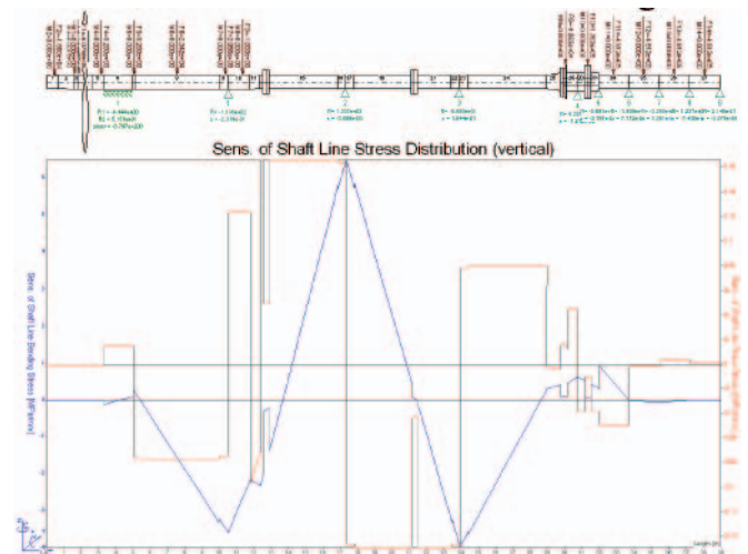
Fig. 15. Influence coefficients of shaft line stresses under the influence of vertical movement of aft intermediate bearing
