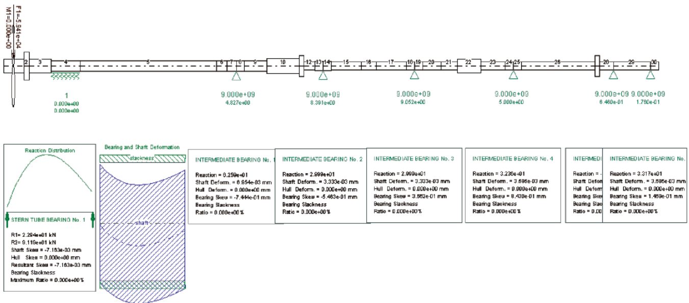
Fig. 18. Shaft line alignment and reactions after correction
