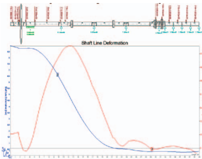
Fig. 10. Modified shaft line deformation
