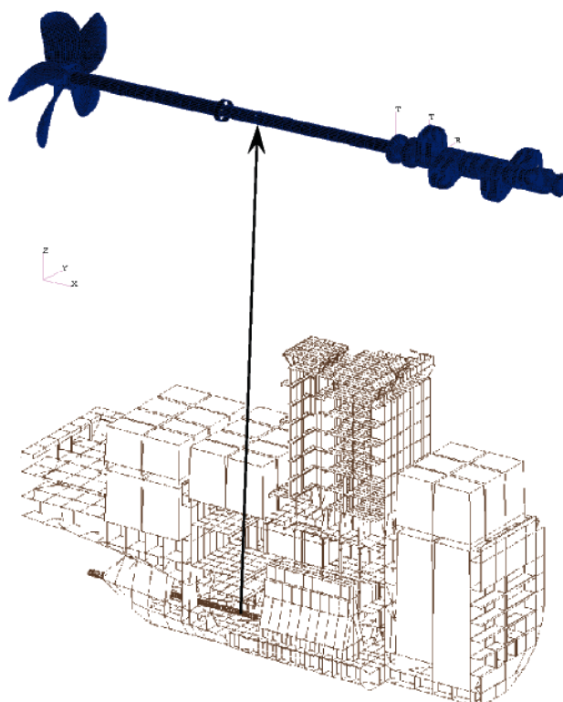
Fig. 1. Typical model of the power transmission system isolated from ship hull
