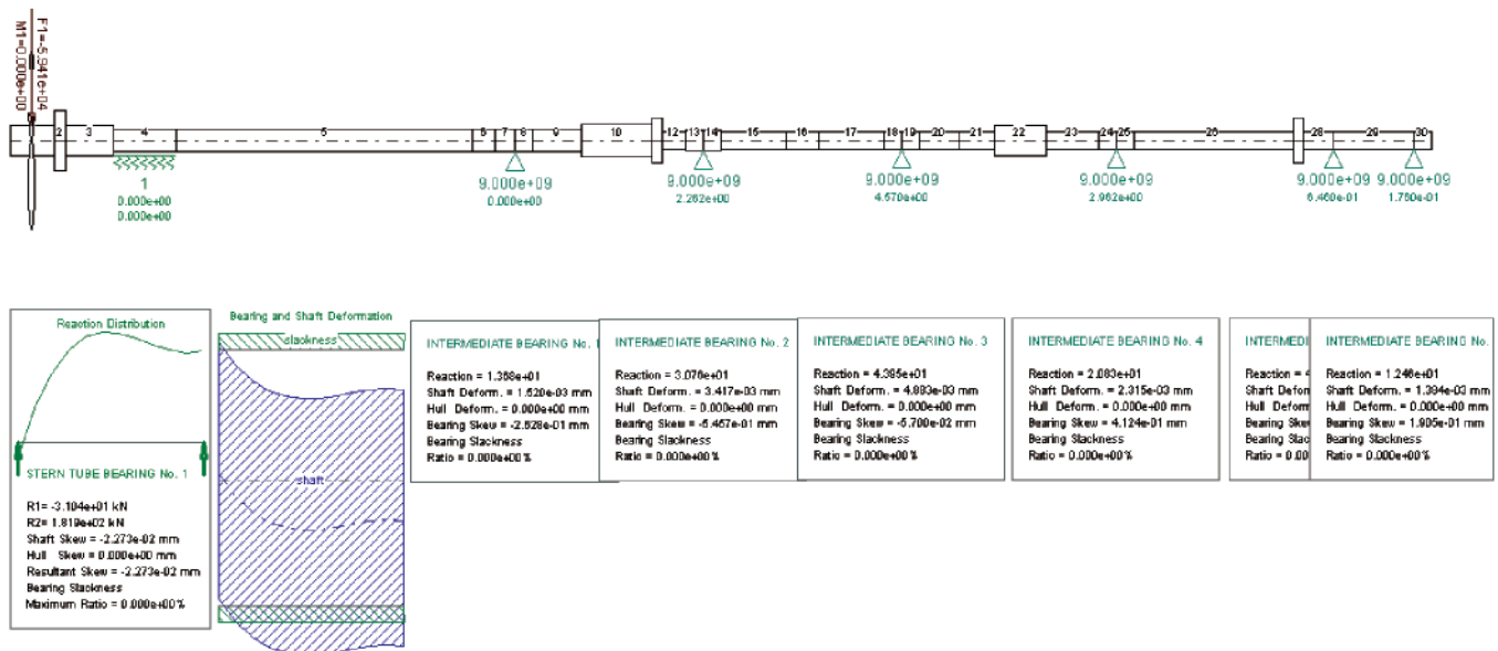
Fig. 17. Real shaft line alignment and reactions
