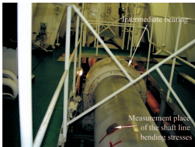
Fig. 2. Bending stress measurement of the shaft line
