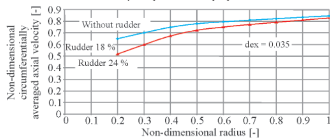
Fig. 6. Influence of the rudders of different thickness on the radial distribution of the circumferential average of the axial component of velocity at propeller location
