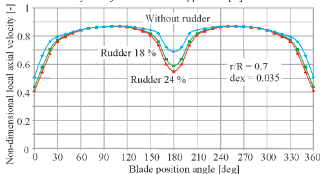
Fig. 5. Influence of the rudders of different thickness on the axial velocity component at the propeller location
