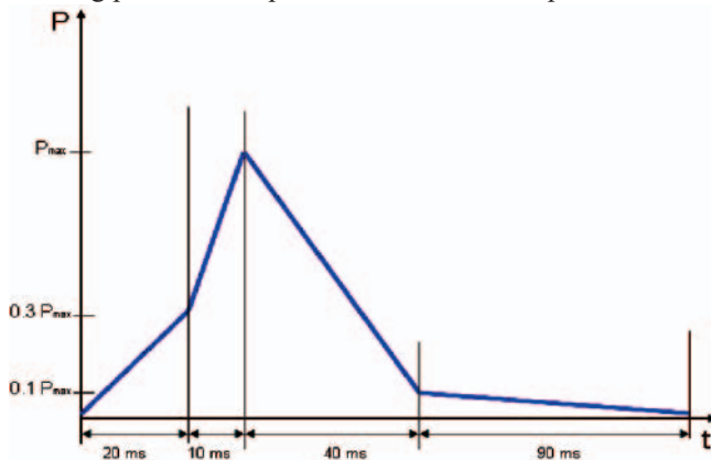
Fig. 2. A design load history for slamming loads on the column face.
