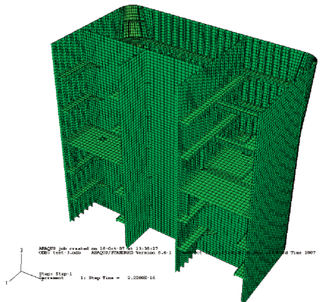
Fig. 5. Cross sectional view of the column
