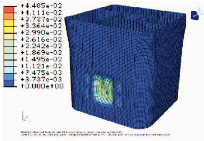
Fig. 8. South wall – exposed area A3, Displacement [m] at Time =50 ms.
