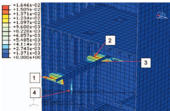
Fig. 9. South wall – exposed area A3, Time =50 ms, PEEQ strains level
