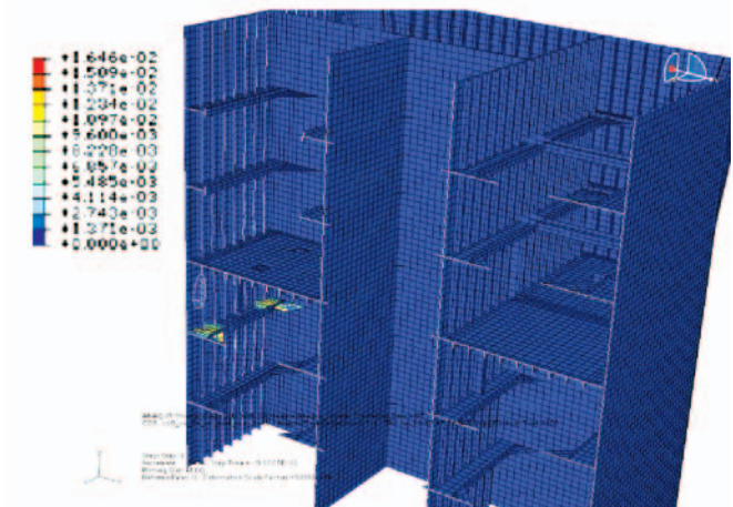
Fig.7. PEEQ strains on south wall of column
