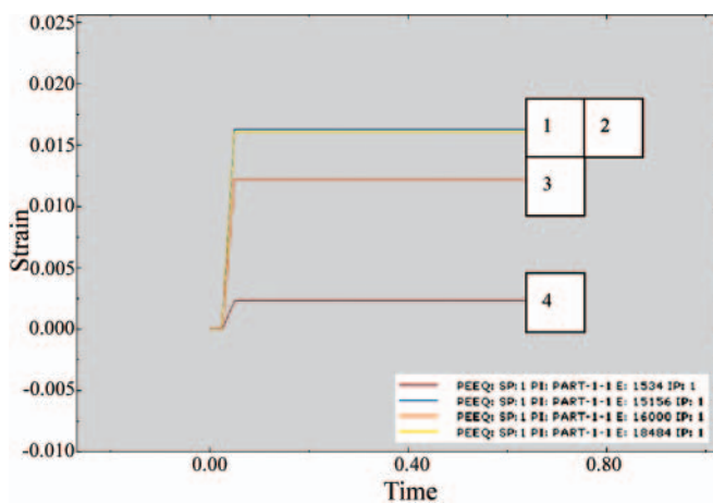
Fig. 10. South wall – exposed area A3. Local plastic equivalent strains (PEEQ) at selected elements as function of time.
