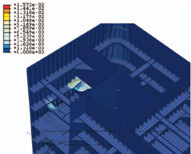
Fig. 6. Von Mises stress distribution from global model load [Pa]
