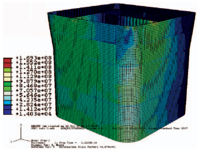
Fig. 6. Von Mises stress distribution from global model load [Pa]
