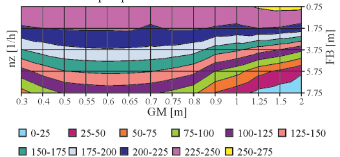
Fig. 7. Statistical hourly occurrence rate of water ingress into the holds, nz , in function of the initial transverse metacentric height GM and the freeboard height FB; for open-top containership of the length L = 144 m, at speed v = 10 m/s, wave encounter angle \beta = 60^\circ , and significant wave height H_s = 8.5 m
