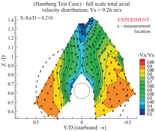
Fig.15. Results of the measurements of axial velocity component, performed on the ship with operating propeller .
