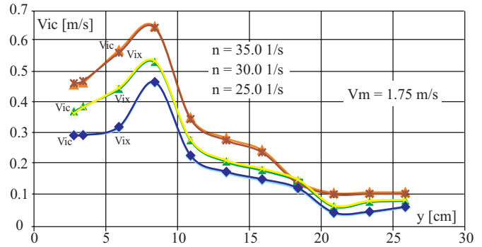
Fig. 13. Axial component and module of propeller-induced velocity measured at the height of the propeller shaft axis of the ship model with the modified stern, at the distance of 157 mm before the propeller .
