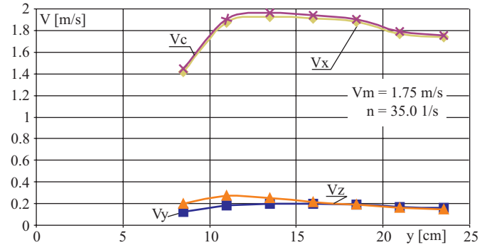
Fig. 8. Velocity components along the measurement line located at the height of the propeller axis, for n = 35 \text{ 1/s} .
