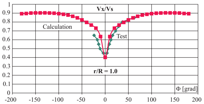
Fig. 17. Comparison of the axial component of before-the-propeller velocity at the radius r/R = 1.0 , obtained from measurements and calculations for the full-scale ship, respectively .
