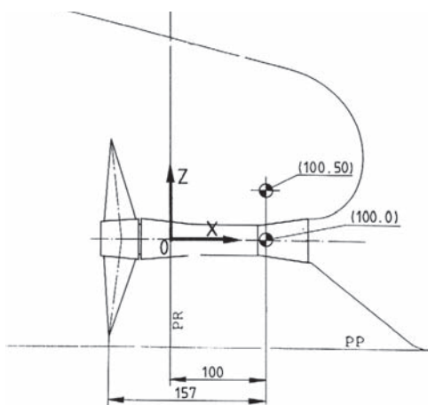
Fig. 12. Location of measurement lines on the ship model with the modified stern. PP - Base plane, PR - Aft perpendicular .
