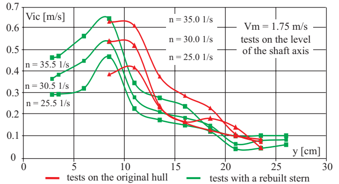
Fig. 14. Comparison of induced velocities obtained from the tests on the models with the original stern and modified one .
