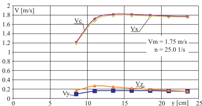
Fig. 6. Velocity components along the measurement line located at the height of the propeller axis, for n = 25 \text{ 1/s} .
