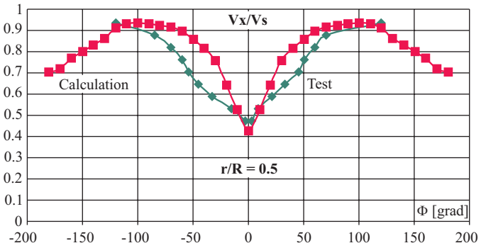
Fig. 19. Comparison of the axial component of before-the-propeller velocity at the radius r/R = 0.5 , obtained from measurements and calculations for the full-scale ship, respectively .
