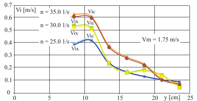
Fig. 10. Axial component and module of propeller-induced velocity along the measurement line located at the height of the propeller shaft axis .
