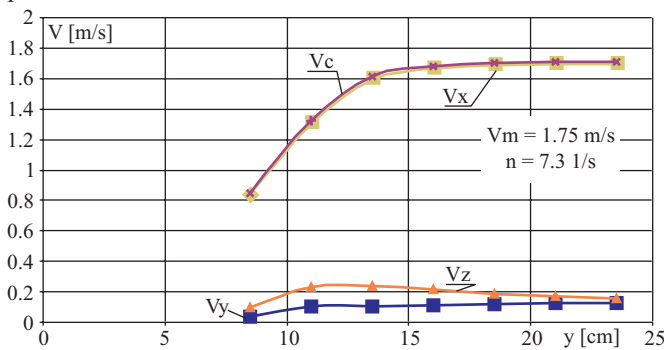
Fig. 5. Velocity components along the measurement line located at the height of the propeller axis, for n = 7.3 \text{ 1/s} (thrust of zero-value) .
