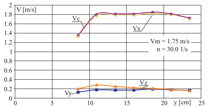
Fig. 7. Velocity components along the measurement line located at the height of the propeller axis, for n = 30 \text{ 1/s} .
