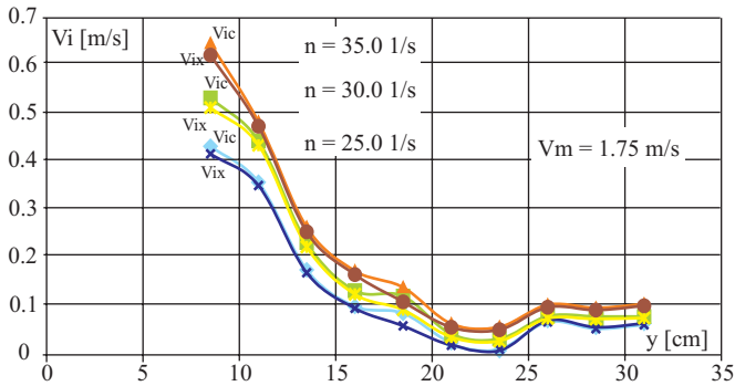
Fig. 11. Axial component and module of propeller-induced velocity along the measurement line located at the height above the propeller shaft axis by 50 mm .
