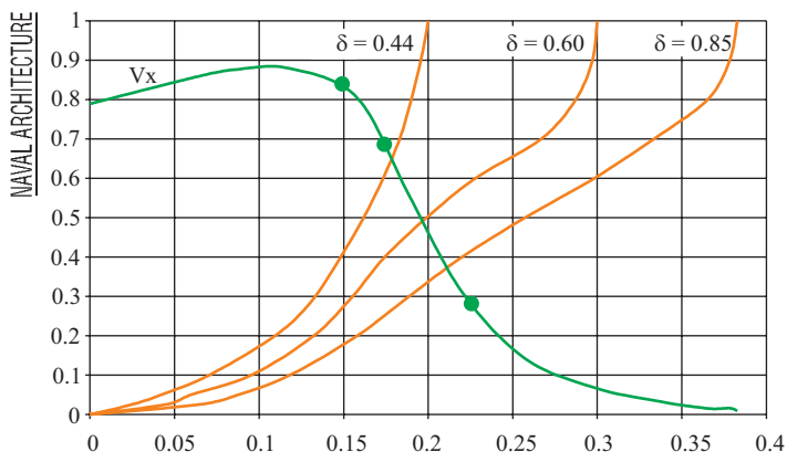
Fig. 2. Distribution of axial component of velocity in before-the-propeller flow, obtained from the original Biot-Savart formula, shown on the background of frame sections of hulls having various block coefficients.
