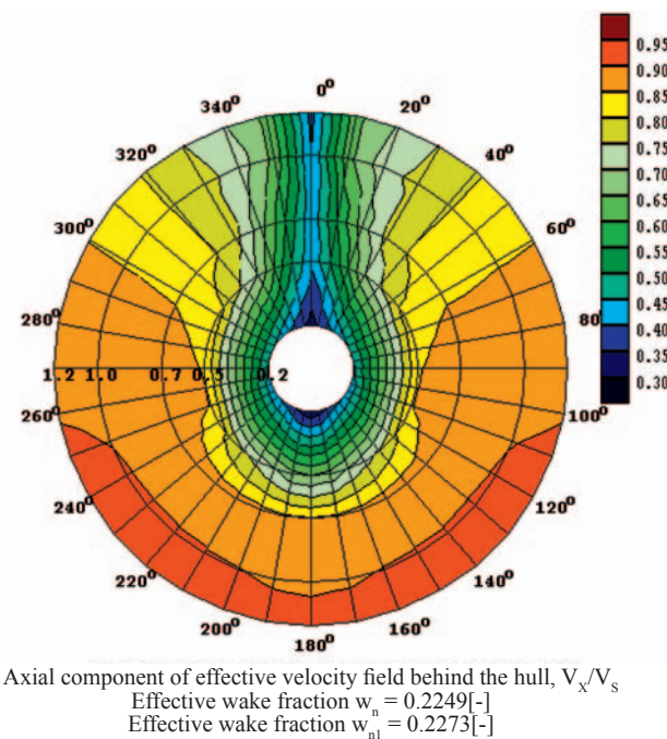
Fig. 16. Results of the measurements of axial velocity component, performed on the ship with operating propeller .
