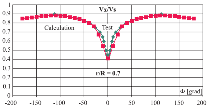
Fig. 18. Comparison of the axial component of before-the-propeller velocity at the radius r/R = 0.7 , obtained from measurements and calculations for the full-scale ship, respectively .
