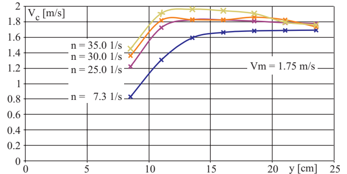
Fig. 9. Modules of velocities along the measurement line located at the height of the propeller axis, for various values of propeller rotational speed .
