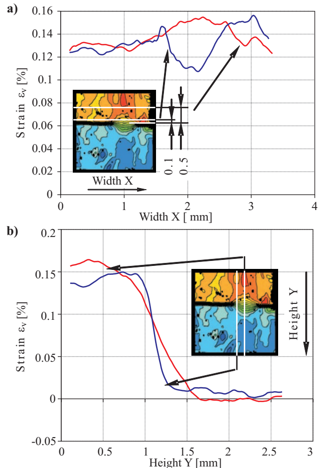
Fig. 6. ( \epsilon_v ) strain distributions in B_1 specimen in load direction : a) along specimen axis and b) transversely to it, for loading force P = 20 kN .
