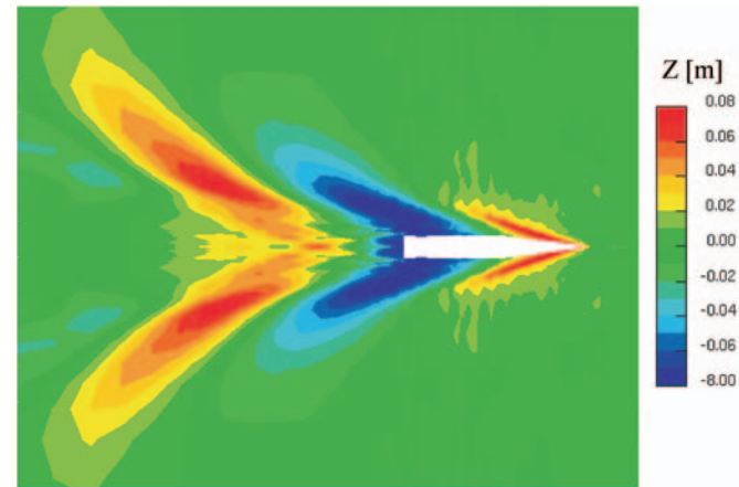
Fig. 19. Wave contour at Froude number F_n = 0.6 .
