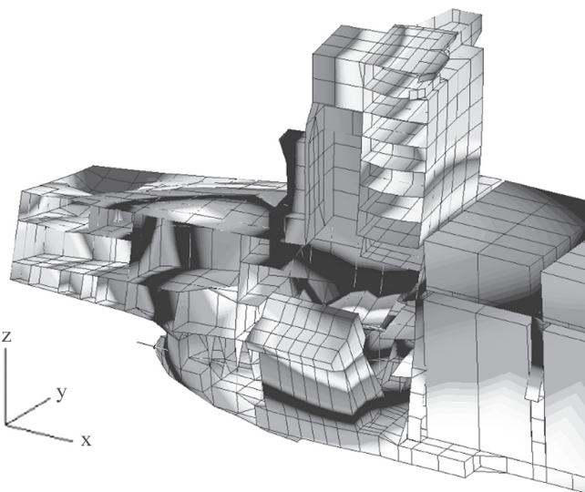
Fig. 9. Vibrations forced by 5 th harmonic component (X type) of main engine's external moments
