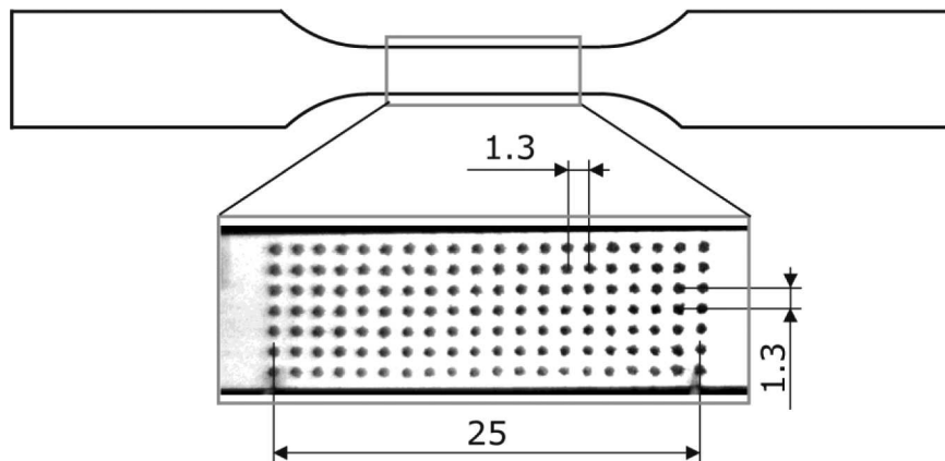
Fig. 2. Markers in form of dots placed on the one side of gauge part of the specimen
