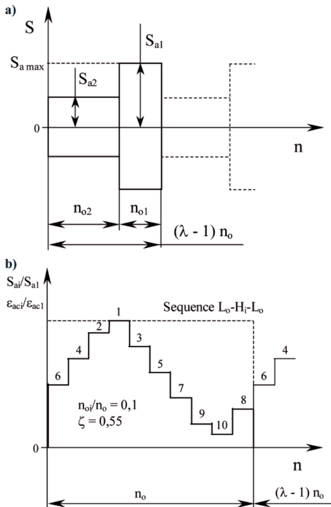
Fig. 1. Schematic diagrams of the load programs assumed for calculations: a) two-level program, b) multi-level program
