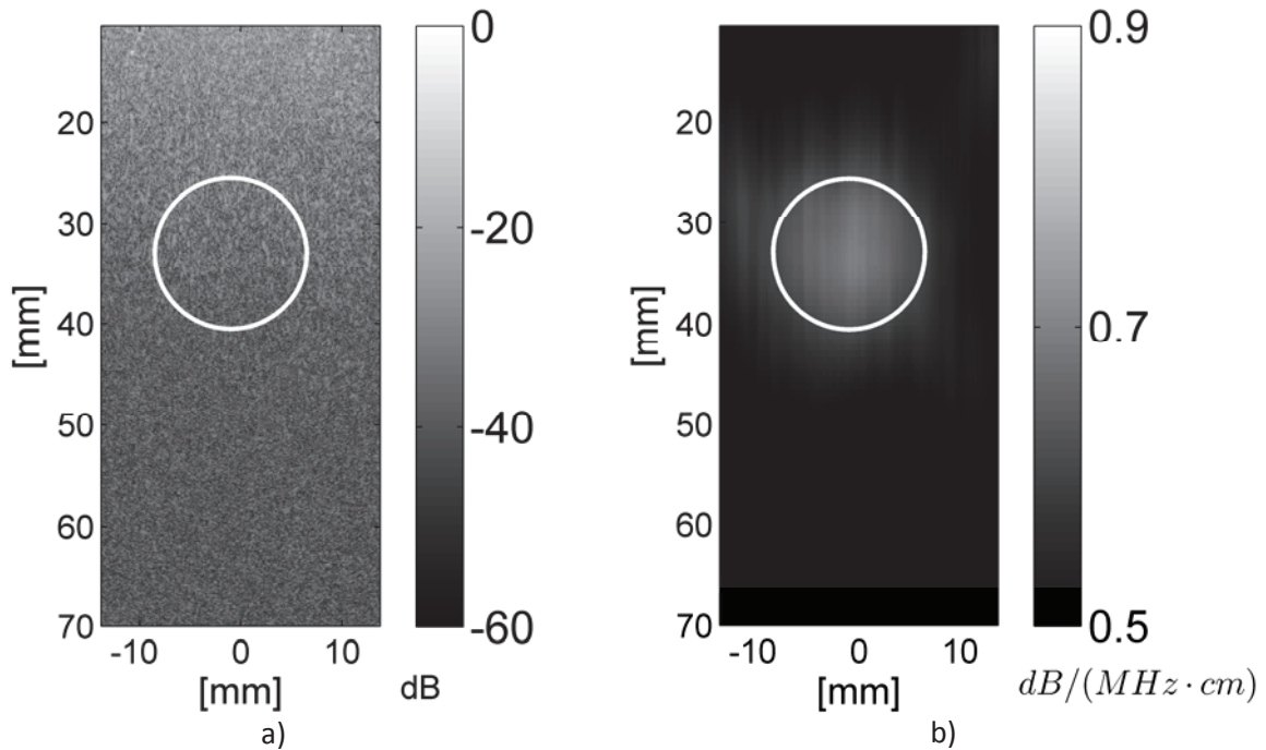
Fig.7. The standard B mode image (a) and the attenuation map (b) present the attenuating object in tissue mimicking phantom. The attenuation of background and the object was equal 0.5 and 0.7 dB/(MHz·cm) respectively.
