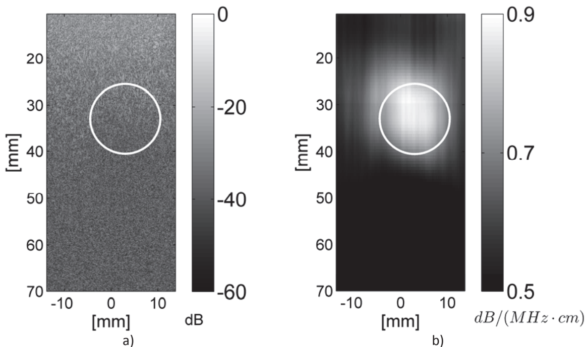
Fig.8. The standard B mode image (a) and the attenuation map (b) present the attenuating object in tissue mimicking phantom. The attenuation of background and the object was equal to 0.5 and 0.9 dB/(MHz·cm) respectively.
