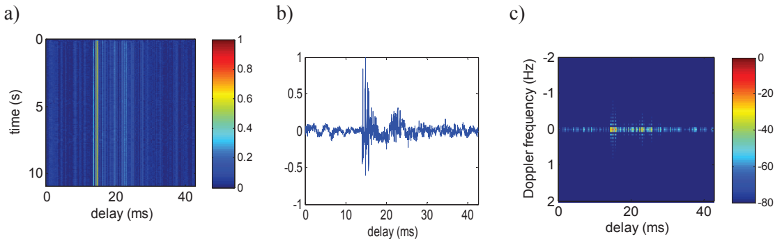
Fig.3. Static acoustic reverberant channel, distance 4.5 m; impulse responses (a), single impulse response (b), and scattering function (c).
