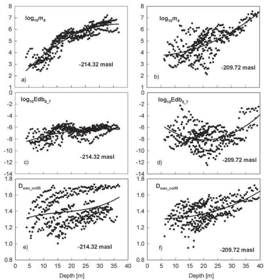
Fig.4. The depth dependences of selected echo parameters along 13 offshore transects (left figures – December, 30, 2002) and 12 transects (right figures – May, 21, 2003). The data were binned using a 0.5-m depth interval, and each point represents the mean of usually 10–100 measurements
