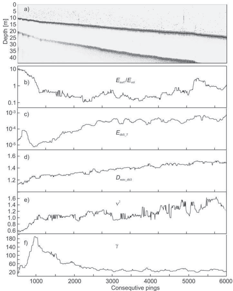
Fig.3. (a) Echogram of the offshore TA transect collected on October 30, 2002. Echo envelope variables: (b) ratio of surface scattering energy to volume scattering energy E_{surf}/E_{vol} , (c) E_{db5_7} - energy of Daubechies wavelet of order 5 and scale a=2^7 , (d) D_{wav\_db3} - fractal dimension computed using Daubechies wavelets of the third order, (e) spectral width - v^2 , (f) spectral skewness - \gamma . TA transect is positioned between Kinneret Limnological Laboratory and lake interior (Fig. 1)
