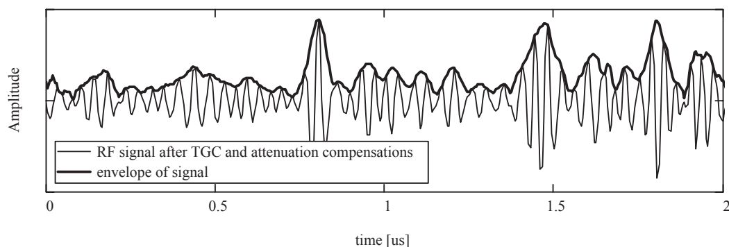
Fig.3. RF signal after the TGC and attenuation compensations and its envelope
