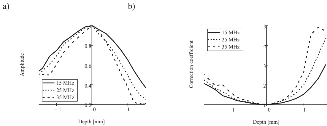
Fig.1. The amplitude of the selected frequency components of the emitted pulse spectrum measured at different depth(a), and corresponding correction curves (b). 0-depth indicates focal plane position
