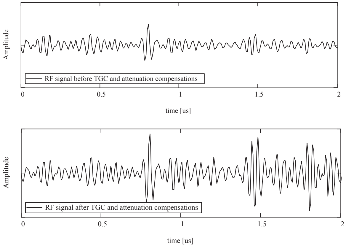
Fig.2. RF signal before (a) and after (b) the TGC and attenuation compensations
