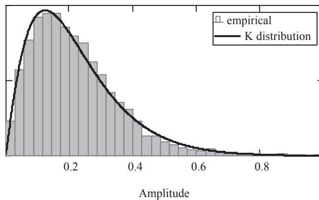
Fig.4a. The comparison of K distribution and empirical data histogram (nape of a neck)
