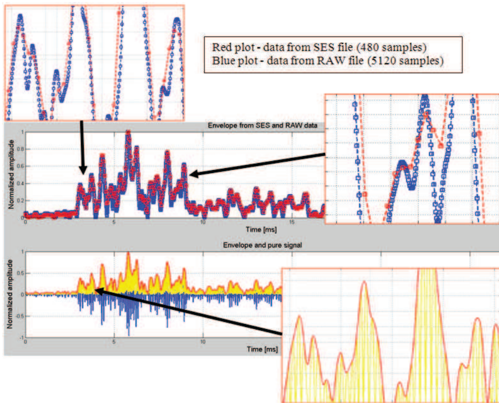
Fig.8. Comparison of *.SES and *.RAW data
