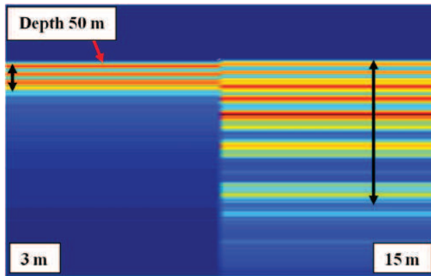
Fig.9. Echogram with minimum threshold value
