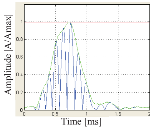
Fig.3. Envelope of received pulse
