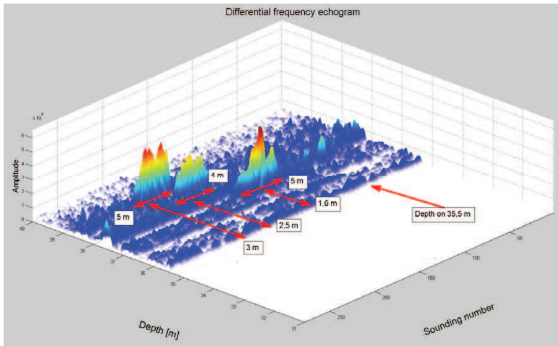
Fig.20. Three buried objects – illustrated in Matlab
