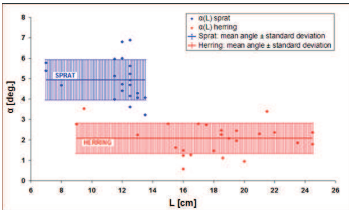
Fig.6. The dependencies of the shift angle \alpha on the total fish length ( L ) for herring and sprat
