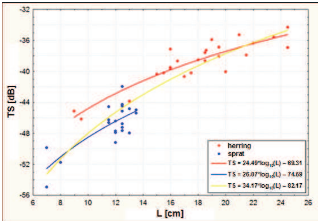
Fig.7. TS(L) dependence for Baltic herring and sprat
