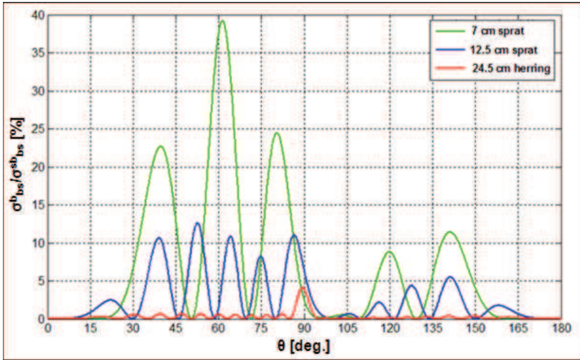
Fig.9. Dependence of the ratio \sigma_{bs}^b / \sigma_{bs}^{sb} on the angle \theta (Figure 1)
