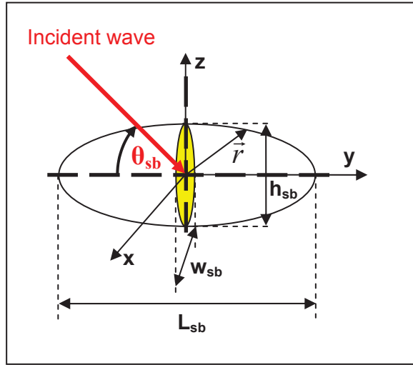
Fig.2. The geometry of the backscattering of acoustic wave at swimbladder
