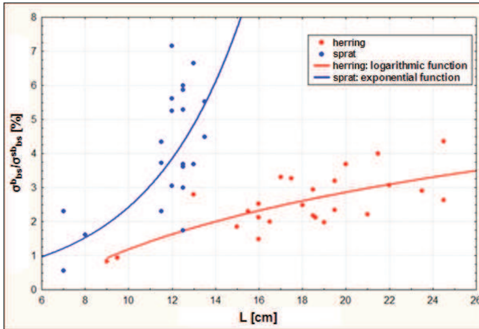
Fig.10. Dependence of the ratio \sigma_{bs}^b / \sigma_{bs}^{sb} on the fish total length (L) for herring and sprat
