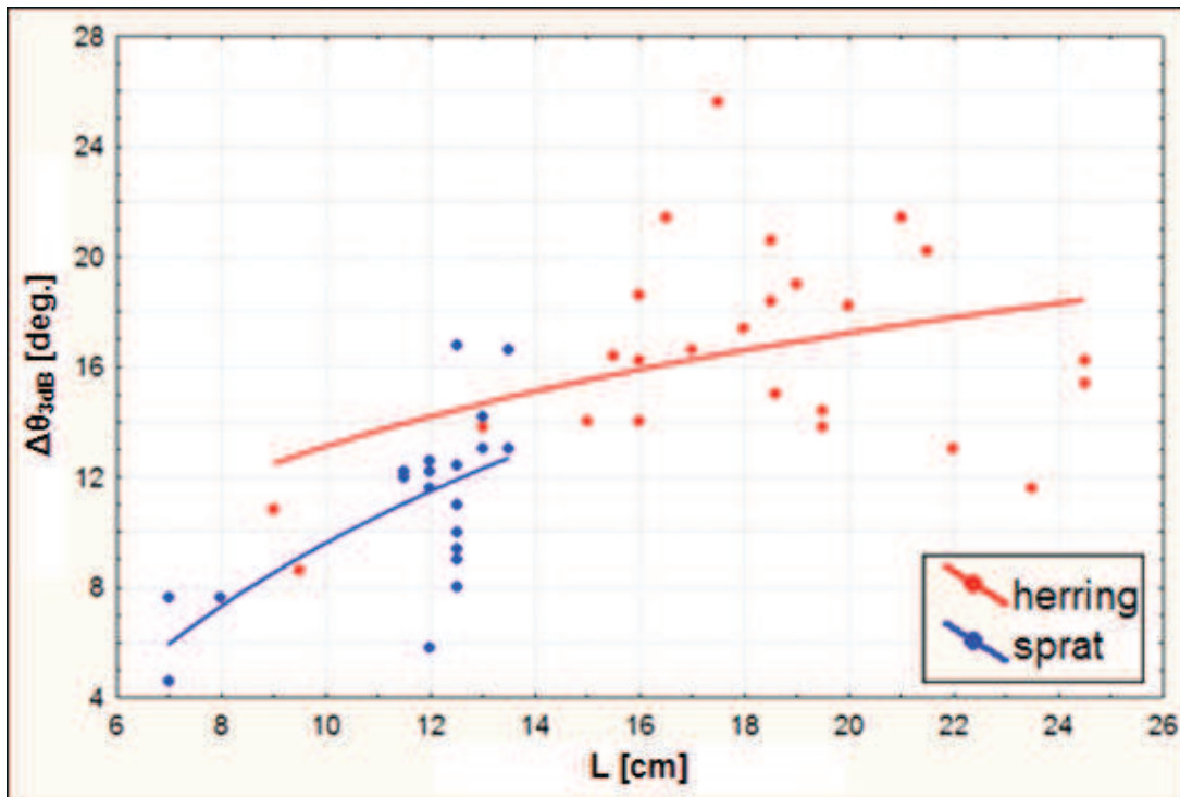
Fig.8. Dependence of the width of directivity function on the total length of fish L
