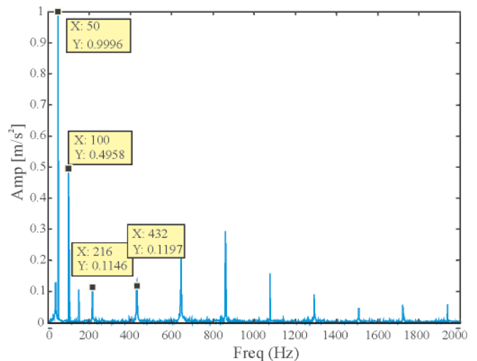
Fig. 2. Frequency spectrum of the vibration signal shown in Fig (1-c), the graph shows vibration amplitude ( m/s^2 ) versus frequency (Hz)
