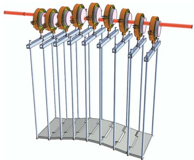
Fig. 2. Detail of the undulating surface and mechanical transmission of movement
