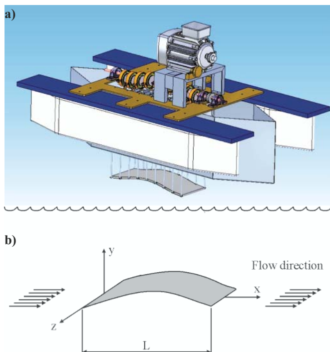
Fig. 1. a) experimental mechanism, b) detail of the fin
