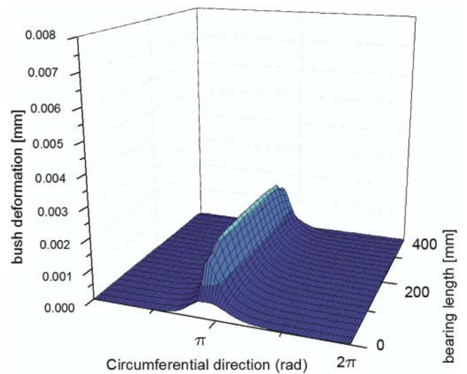
Fig. 10. The calculated bush surface deformation in a highly loaded sliding bearing with stiff composite bush; for shaft diameter of 100 [mm], diameter clearance of 0.4 [mm], lubricating film thickness of 5 [μm]
