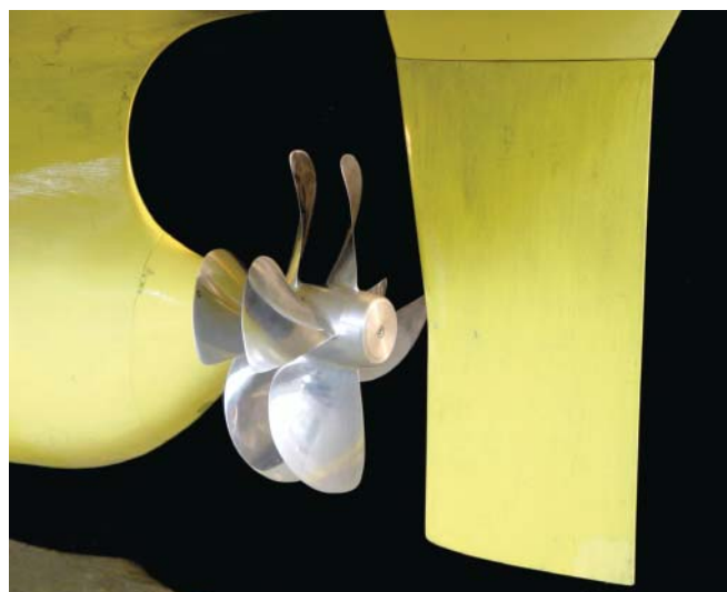
Fig. 1. A typical tandem co-rotating propeller (Model tests in the Ship Hydromechanics Division of CTO SA)
