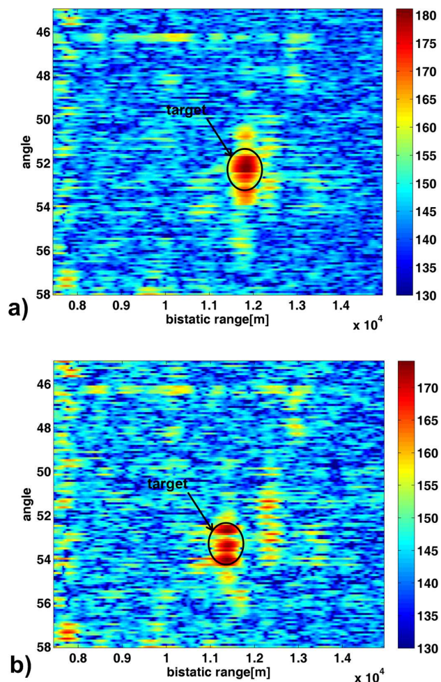
Fig. 11. Results of ground clutter removal for registered data for: a) first Tx antenna beam scan, b) second TX antenna beam scan.
