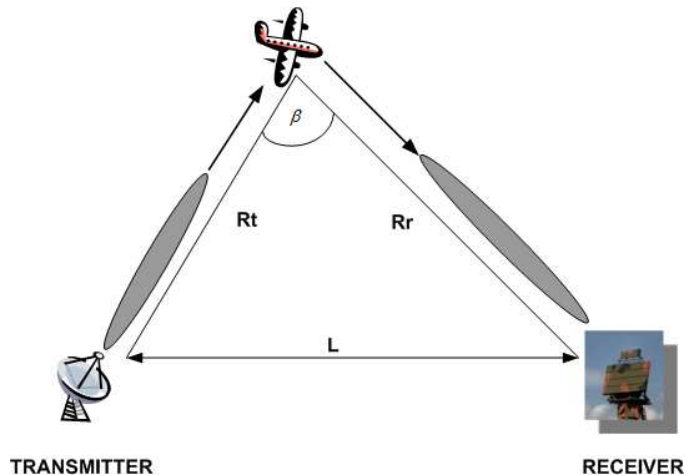
Fig. 1. Simplified bistatic radar geometry.
