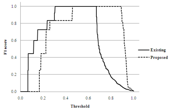
Fig. 6. F1 score for majority of published methods and proposed method.
