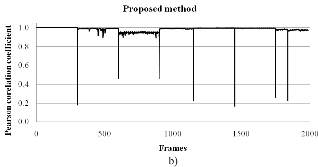
Fig. 5. Shot cut detection by Pearson correlation coefficient for (a) majority of published methods and (b) proposed method.
