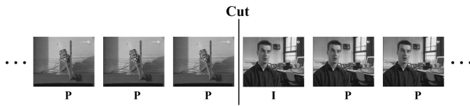
Fig. 4. The principle of proposed adaptive GOP structure.
