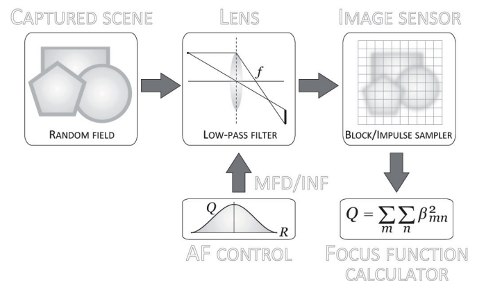
Fig. 1. The block diagram of the considered AF system
